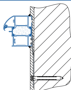
With screw-in anchor
