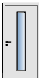
MZ Thermo 46 – TPS 021S Laminated safety glass for exterior, Satinato single-pane safety glass for interior, clear view 146 × 1594 mm
