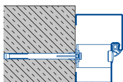
Plug-and-screw fitting
