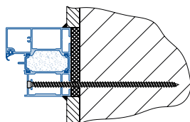
Through-bolt fixing with frame screw (drill holes on-site)
