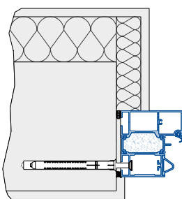
Through-bolt fixing (drill holes on-site)
