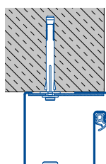
Plug-and-screw fitting
