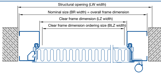
Corner and counter frame with anchor (plug-and-screw fitting)
