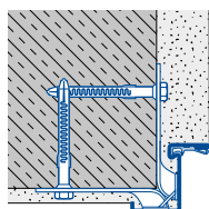
Corner frame with anchor (plug-and-screw fitting)
