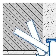
Corner frame with anchor (fix into the wall)
