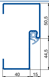
Corner frame with anchor (plug-and-screw fitting)
