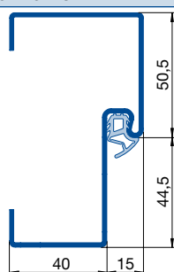
Corner frame with anchor (plug-and-screw fitting, standard)
