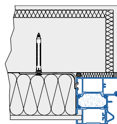
Fitting with screw-in anchor (Plug-and-screw fitting)
