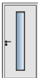
MZ Thermo65 – THP 021S Laminated safety glass for exterior, float glass, Satinato single-pane safety glass for interior, clear view 146 × 1594 mm
