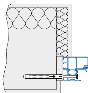
Through-bolt fixing (drill holes on-site)
