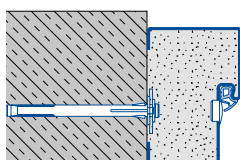
Plug-and-screw fitting
