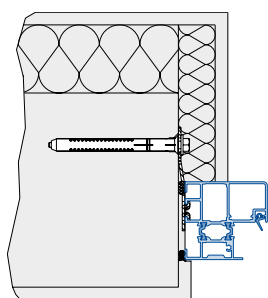
Fitting with screw-in anchor (Plug-and-screw fitting)
