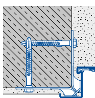
Corner frame with anchor (plug-and-screw fitting, standard)
