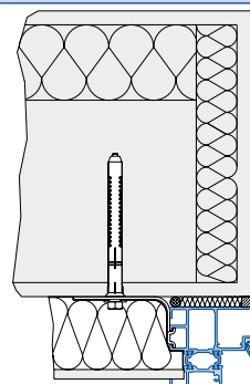
Fitting with screw-in anchor (Plug-and-screw fitting)
