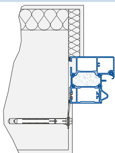
Fitting with screw-in anchor (Plug-and-screw fitting)
