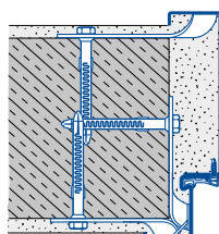
Corner and counter frame with anchor (plug-and-screw fitting)
